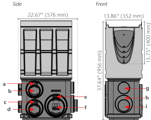
K2-621 (K200) part no. 94620
