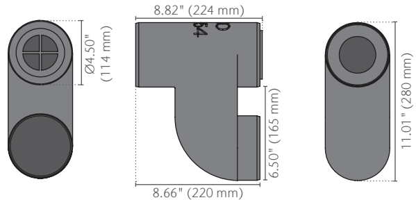
Foul Air Trap (optional) part no. 90854
