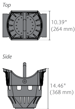
Trash Bucket included with K2-621
